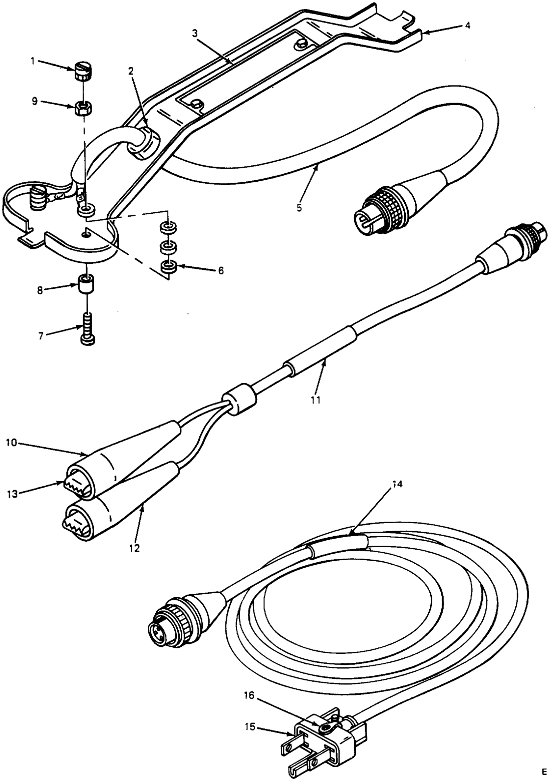
Figure 11. Cable Assemblies CX-1 1964/U, CX-1 1972/U, and CX-1 1971/U
