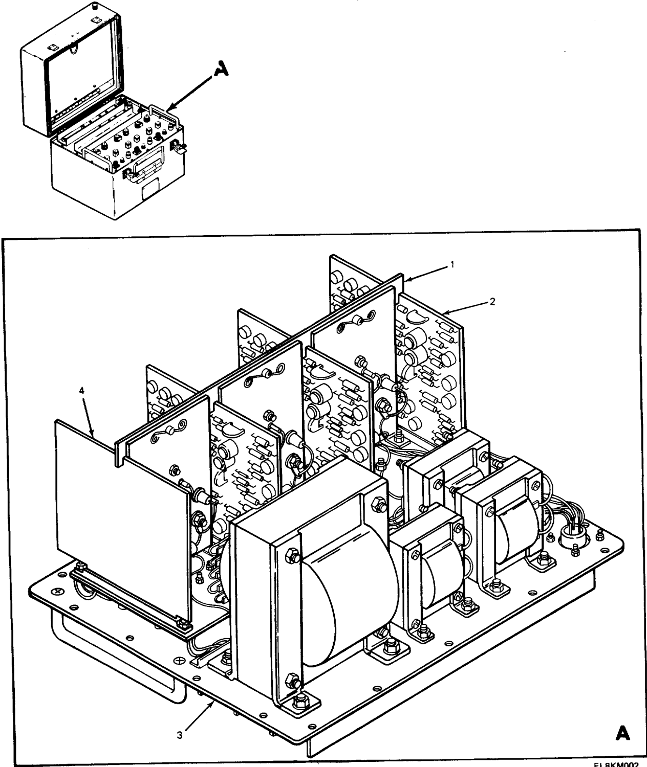
Figure 2. Battery Charger Assembly
