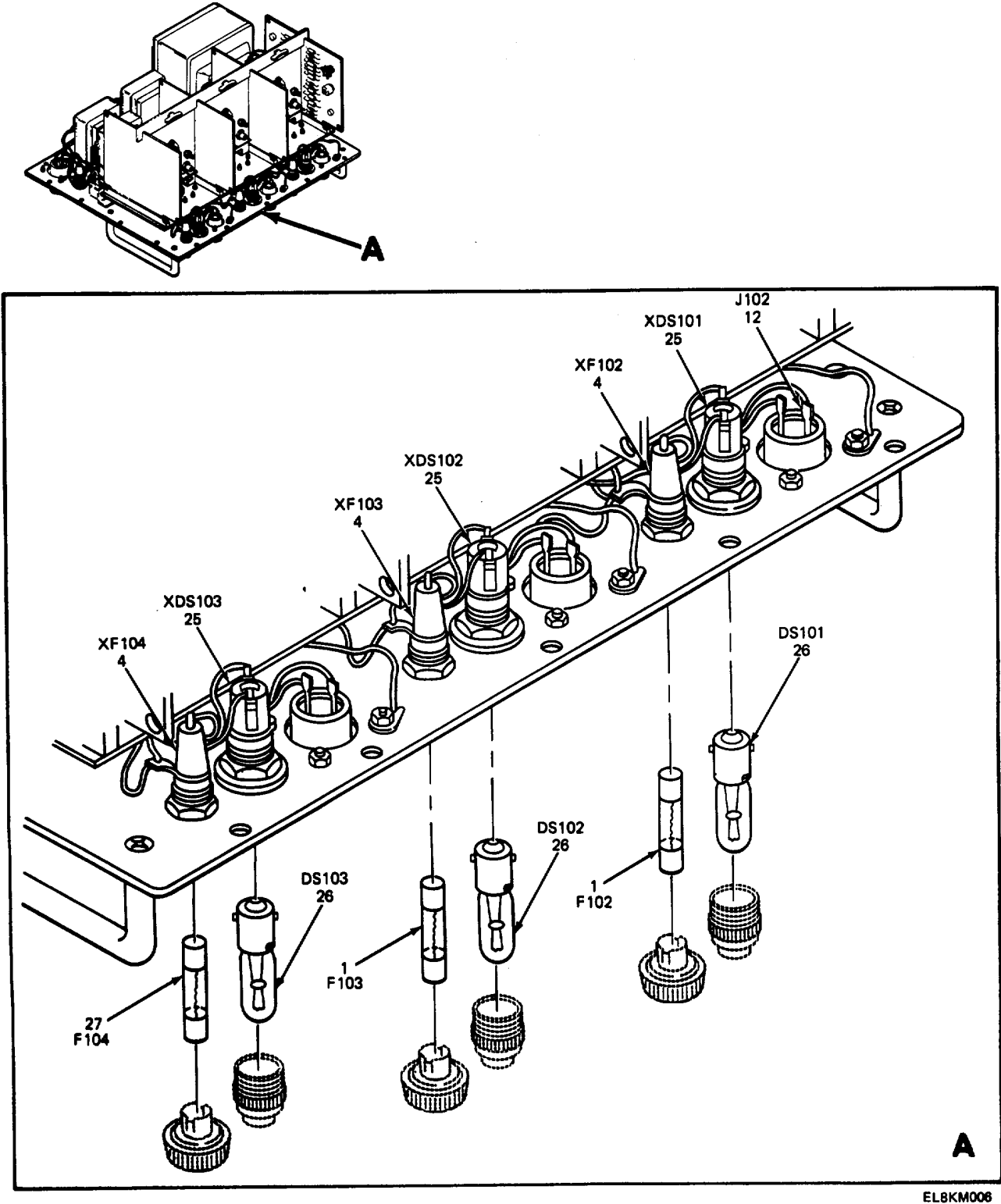
Figure 3. Panel Assembly (Sheet 4 of 4)
