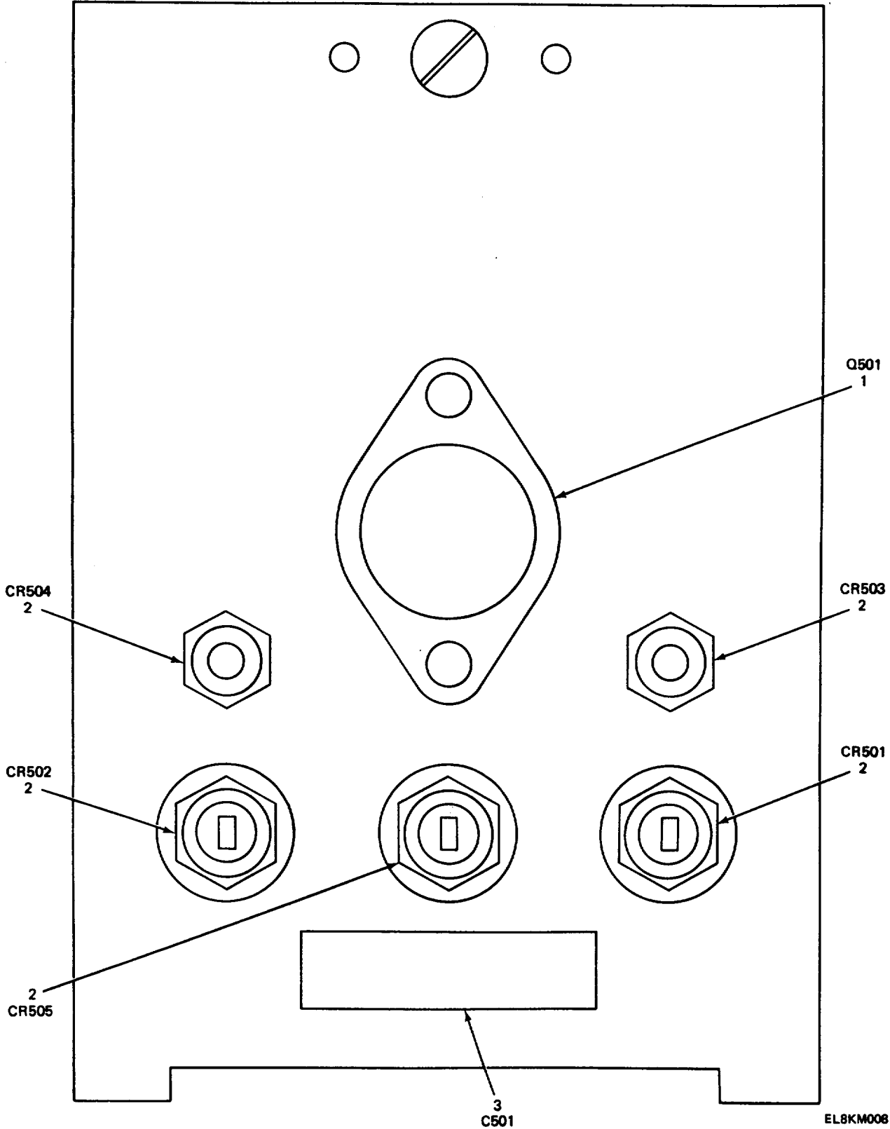
Figure 5. Heat Sink Bracket Assembly
