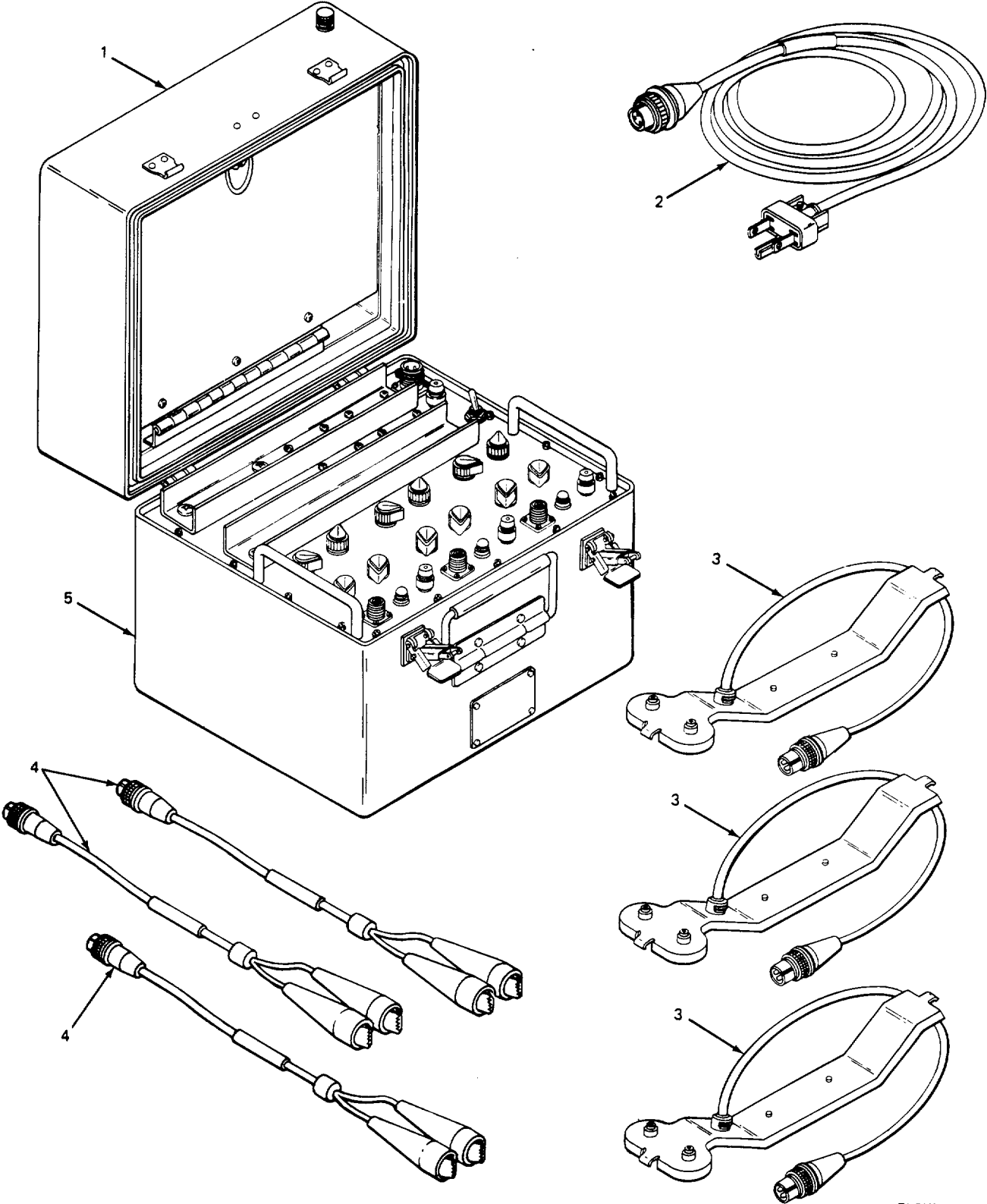
Figure 1. Battery Charger PP-6241/U
