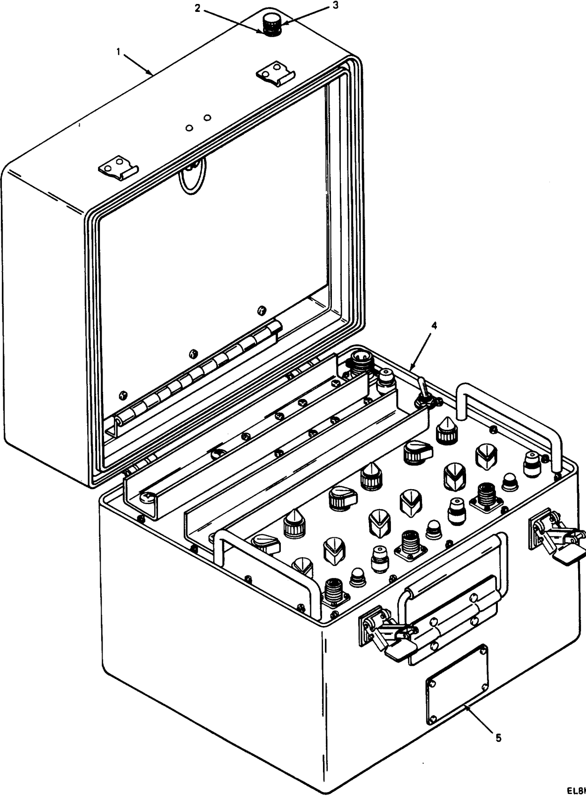
Figure 9. Battery Charger Case Subassembly
