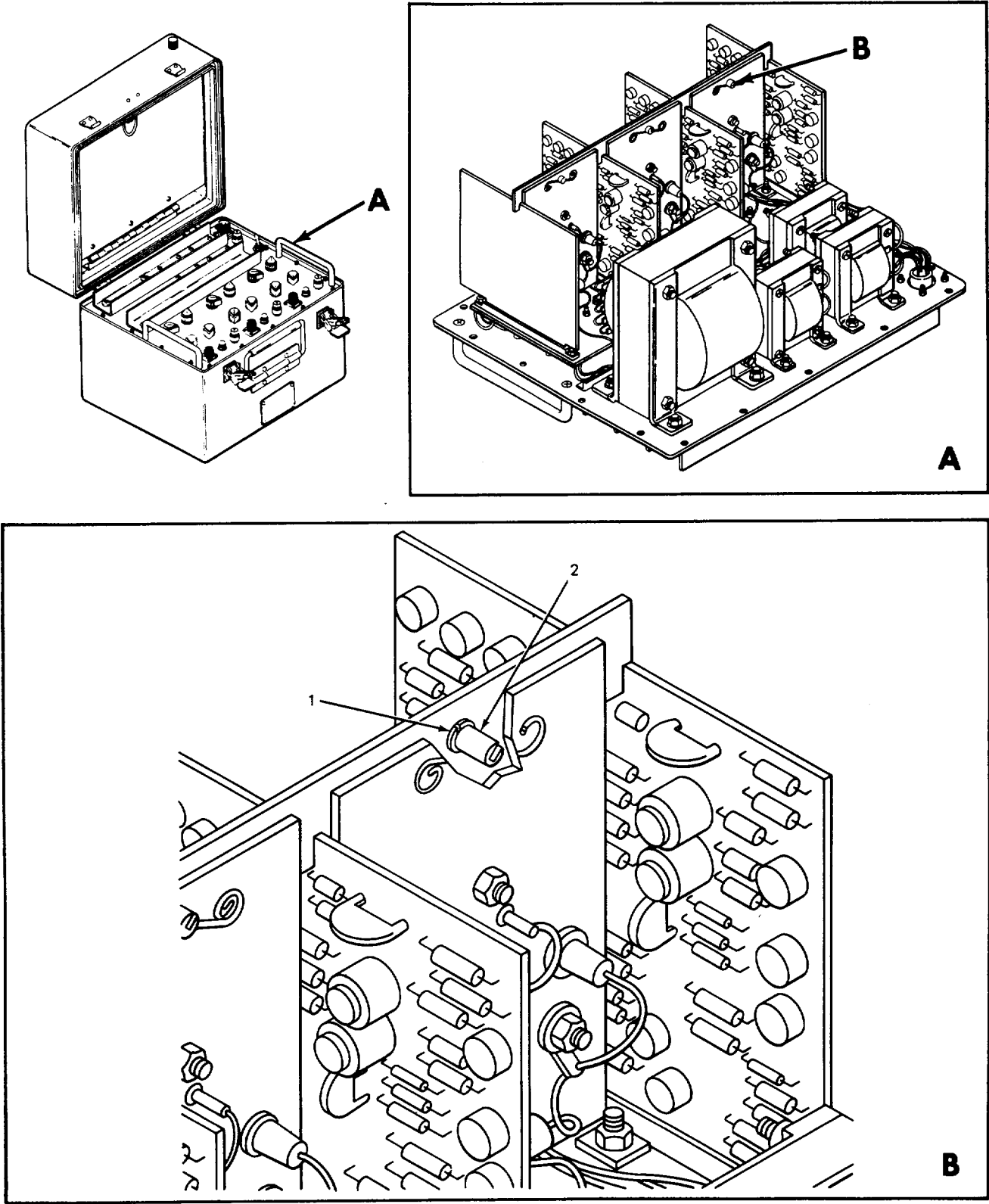
Figure 8. Retainer Assembly
