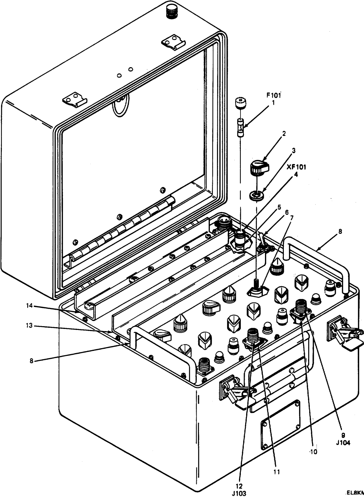
Figure 3. Panel Assembly (Sheet 1 of 4)
